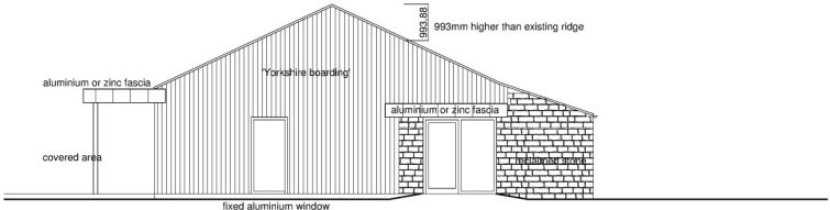
EAST ELEVATION
