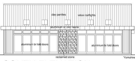
SOUTH ELEVATION
